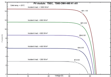
IV Curve
