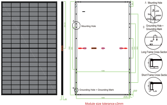
Engineering Drawing(mm)
