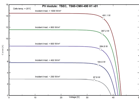
IV Curve
