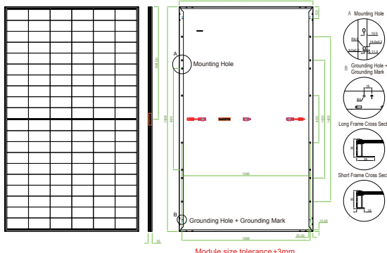
Engineering Drawing(mm)
