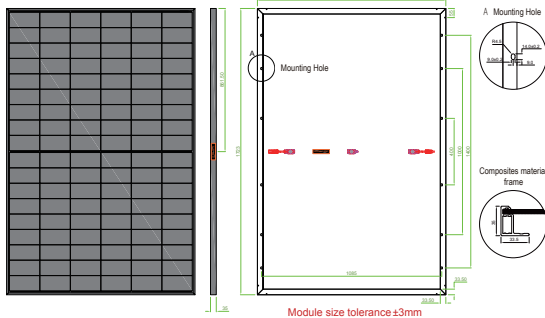
Engineering Drawing(mm)
